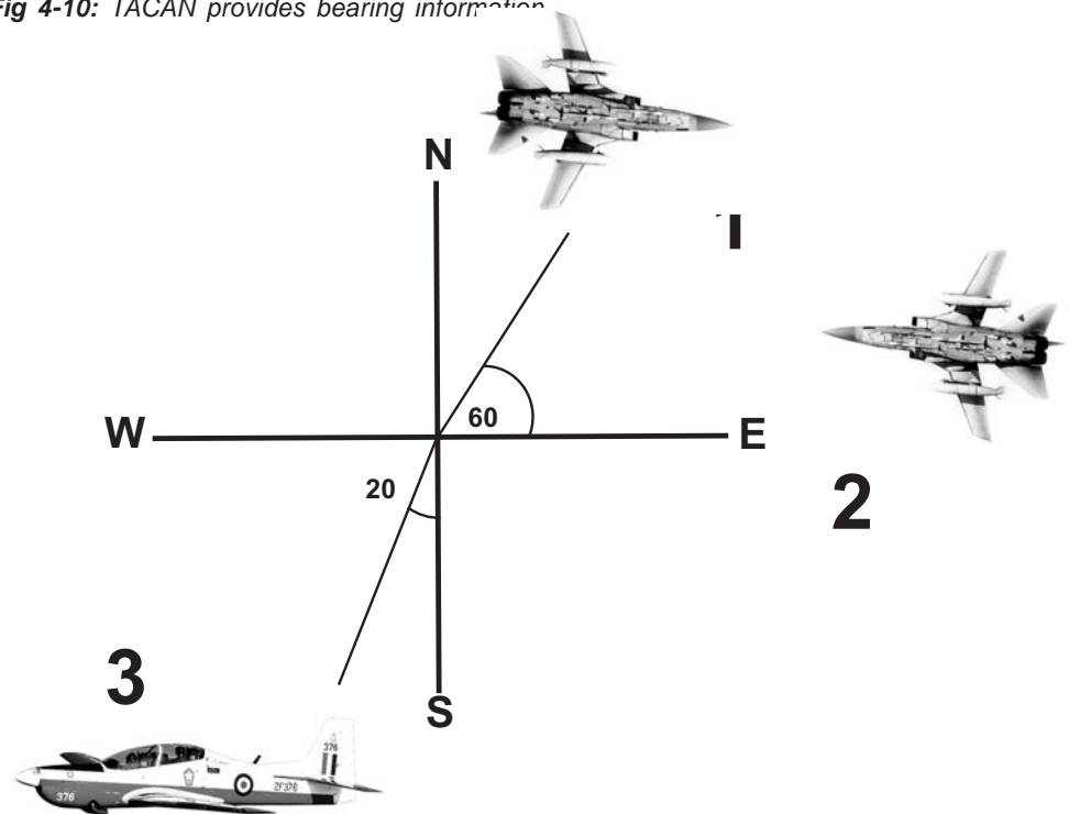
Fig 4-10: TACAN provides bearing information
